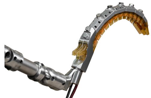
Fig 2. Cutsforth™ Shaft Grounding Assembly: Series 3 that integrates with the Assurance Monitoring System
